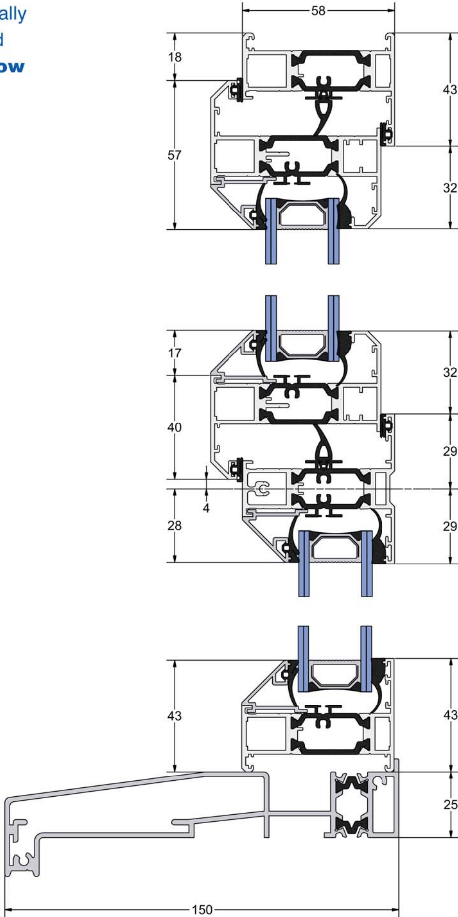
Typical General Arrangement Shown - Not to Scale
